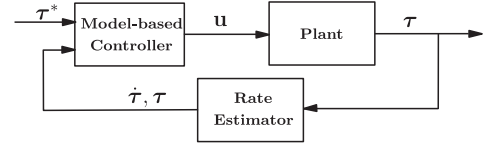
Fig. 5. Schematic representation of the model-based controller.
