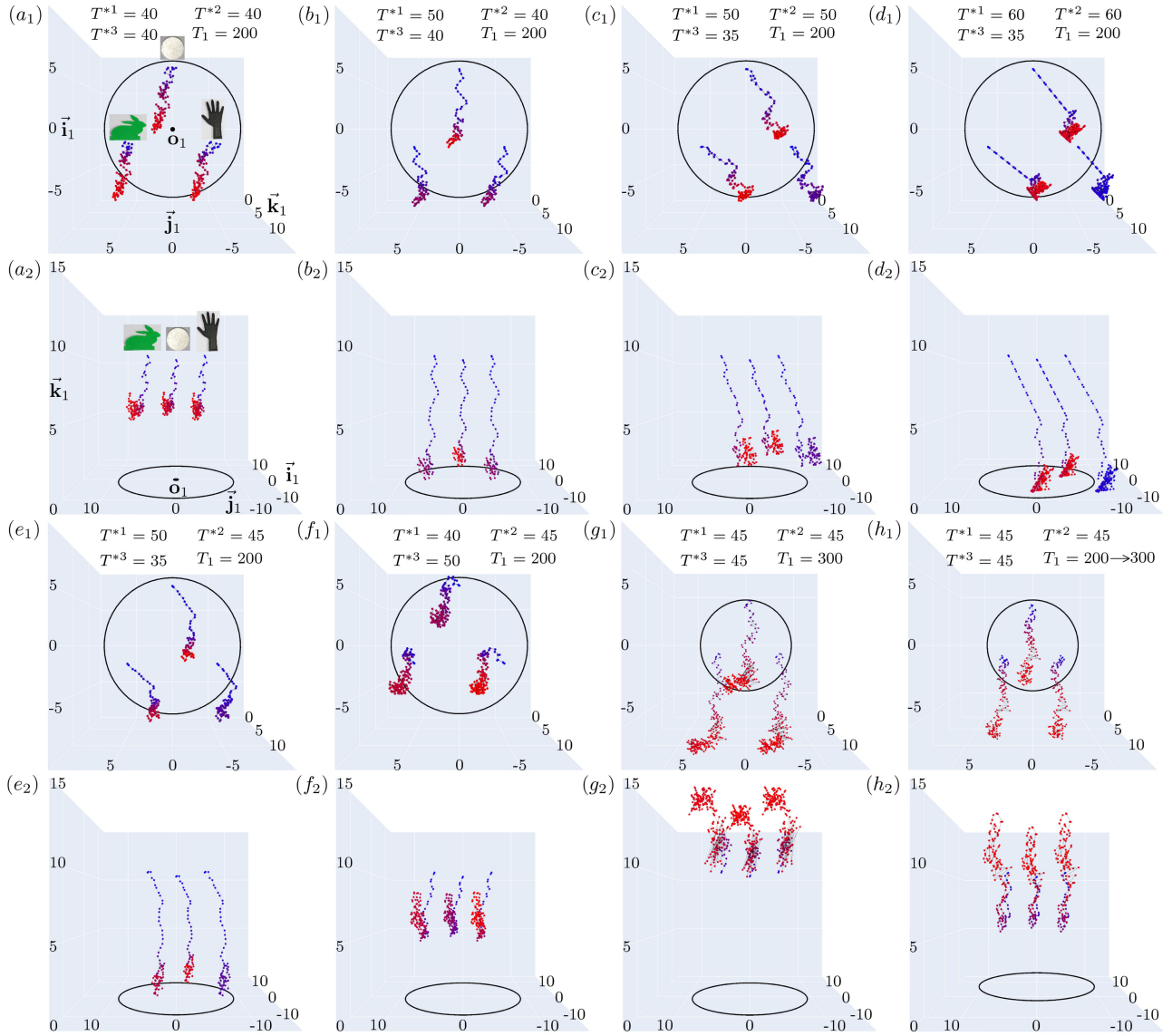
Fig. 13. Spatial displacements of the three objects in the eight experiments with the adaptive controller visualized from two viewing angles. We use a blue-to-red color gradient to visualize the cold-to-hot change of temperatures during the experiments.
