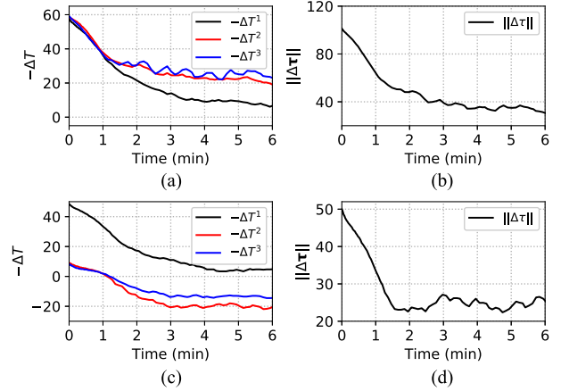
Fig. 16. Evolution of the temperature errors with unfeasible target temperatures: (top) \tau^* = [80, 80, 80]^\top °C, and (bottom) \tau^* = [70, 35, 35]^\top °C.
